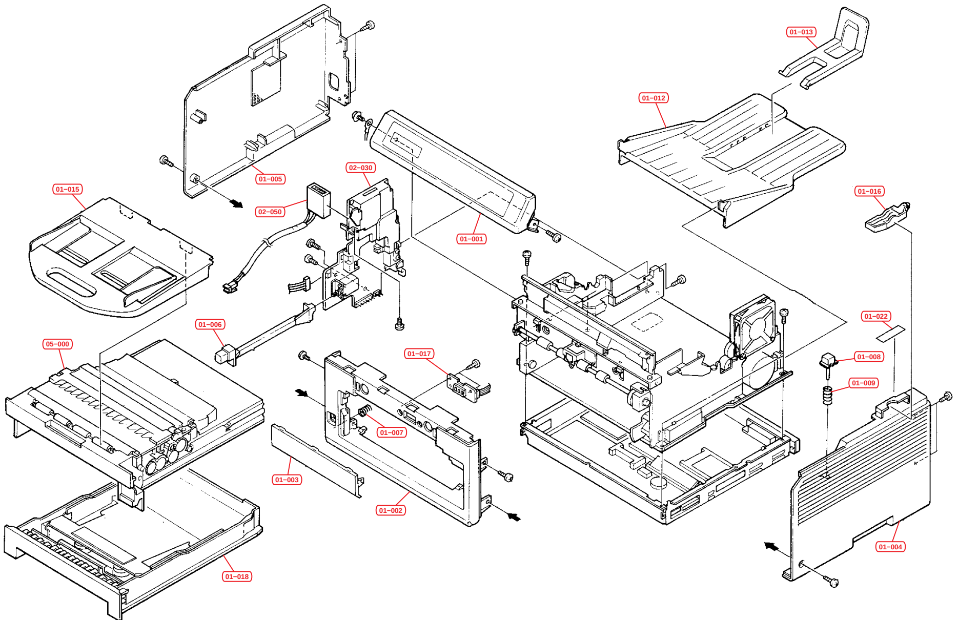
Fig.1 – Covers
