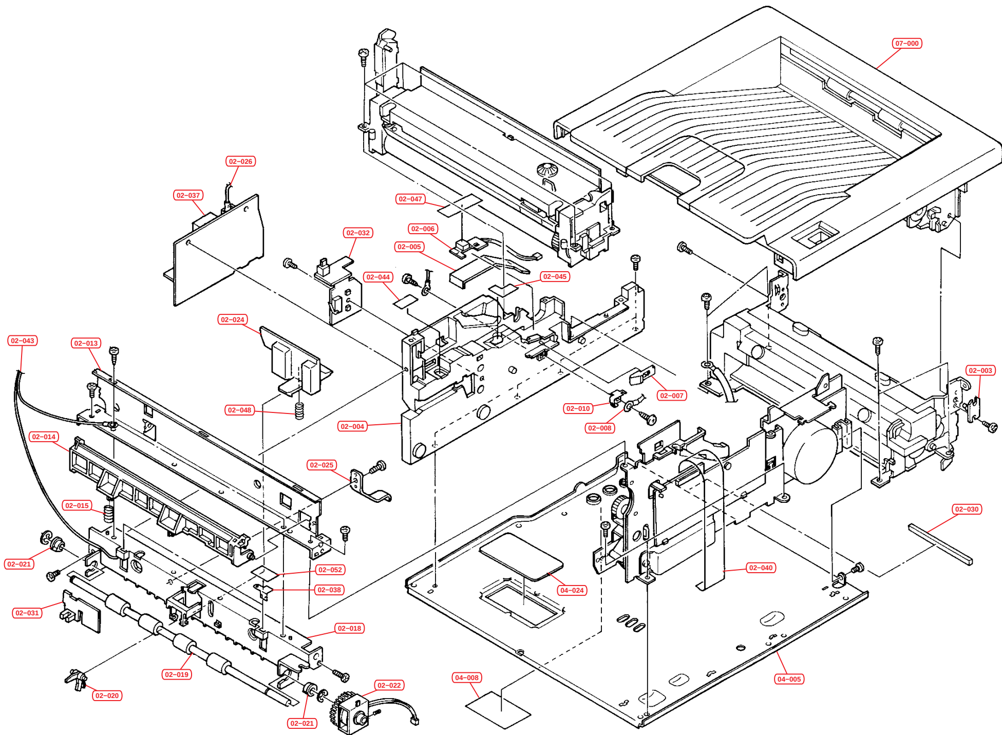
Fig.2 – Frame Unit
